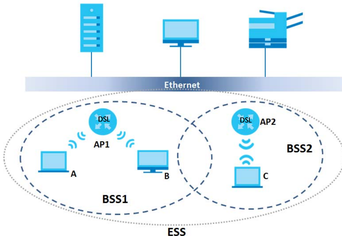
Figure 182 Infrastructure WLAN
